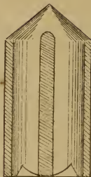
SHAPE OF THE FORE-PART OF THESE BALLS BEFORE FIRING. SHAPE AFTER FIRING.
